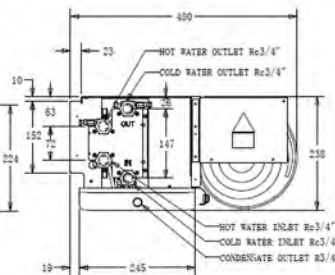
3-1 ROW COIL
