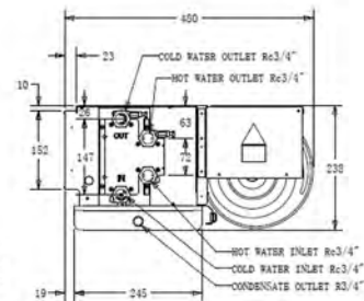
2-1 ROW COIL
